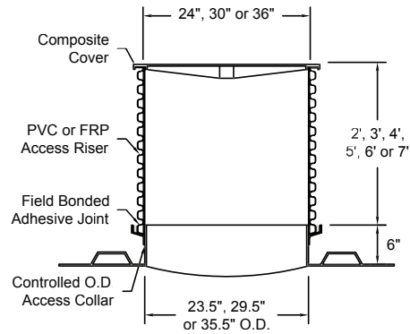
PVC Access Riser with Composite Lid
