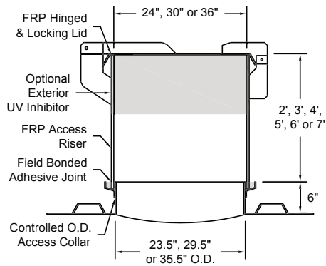
FRP Access Riser with Hinged & Locking Lid
