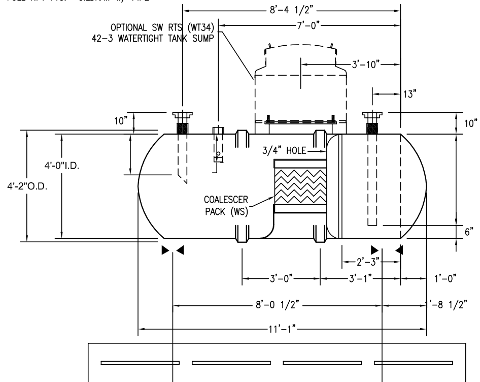
OPTIONAL 18" x 8" x 14' DEADMAN
